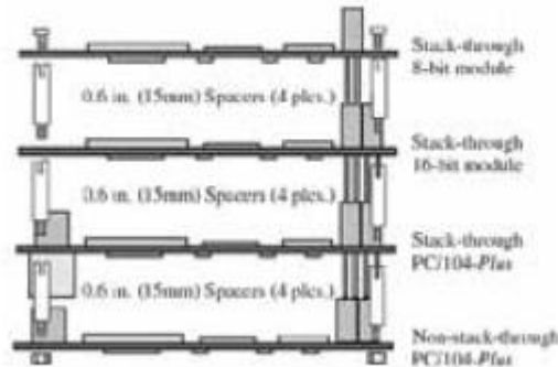
Figure 1: A Possible Module Stack Configuratuin
